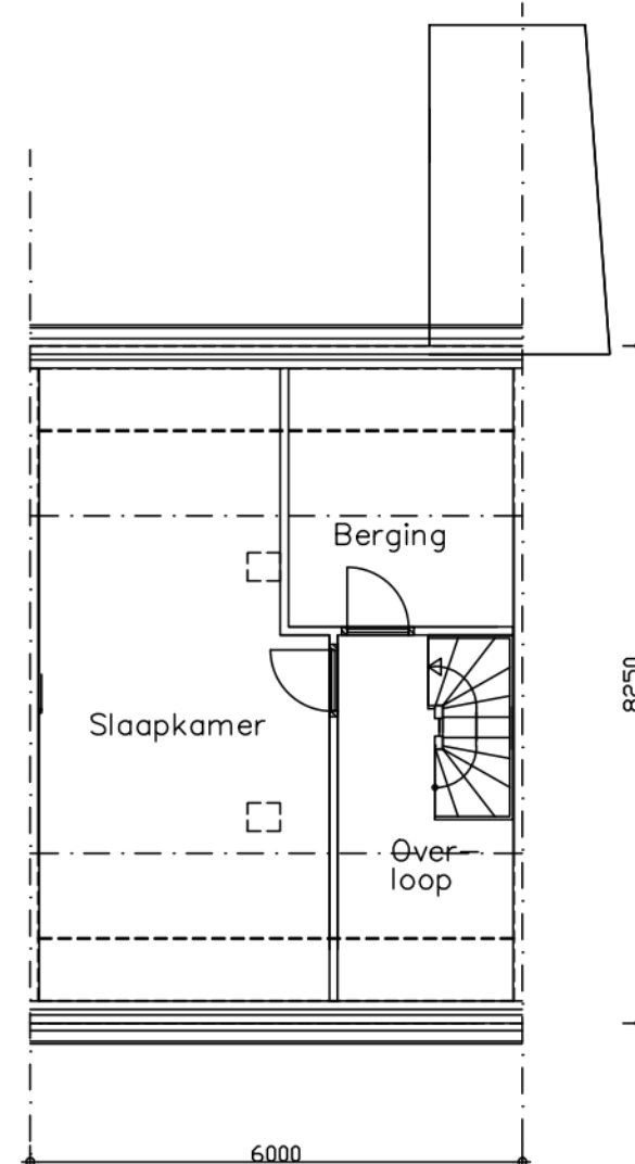
Zolder
