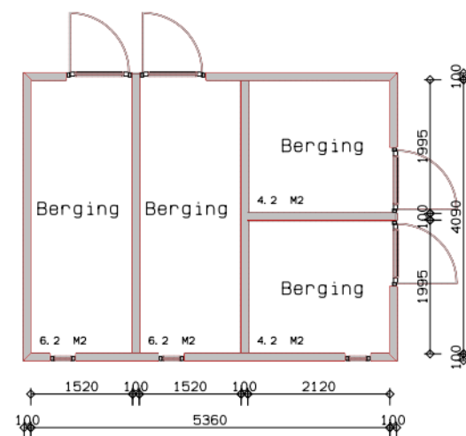
Berging
