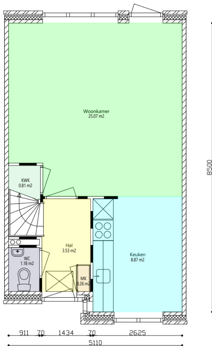
Begane_grond
