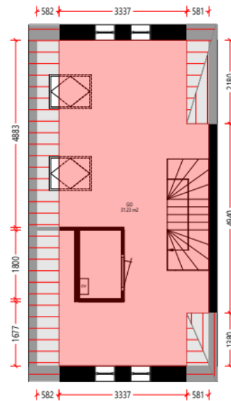
Zolder
