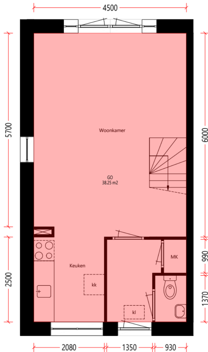
Begane_grond
