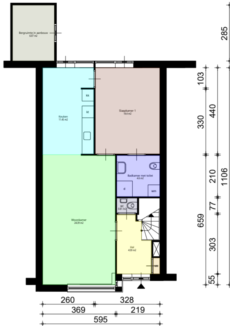
Begane_grond
