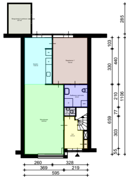
Begane_grond
