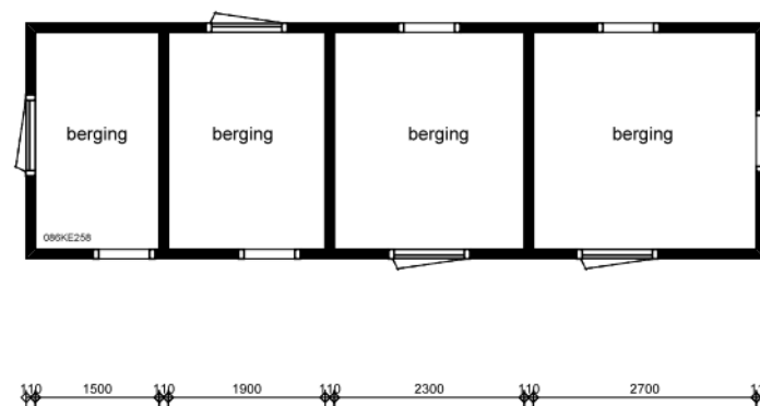
BERGING
