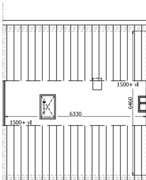
Zolder
