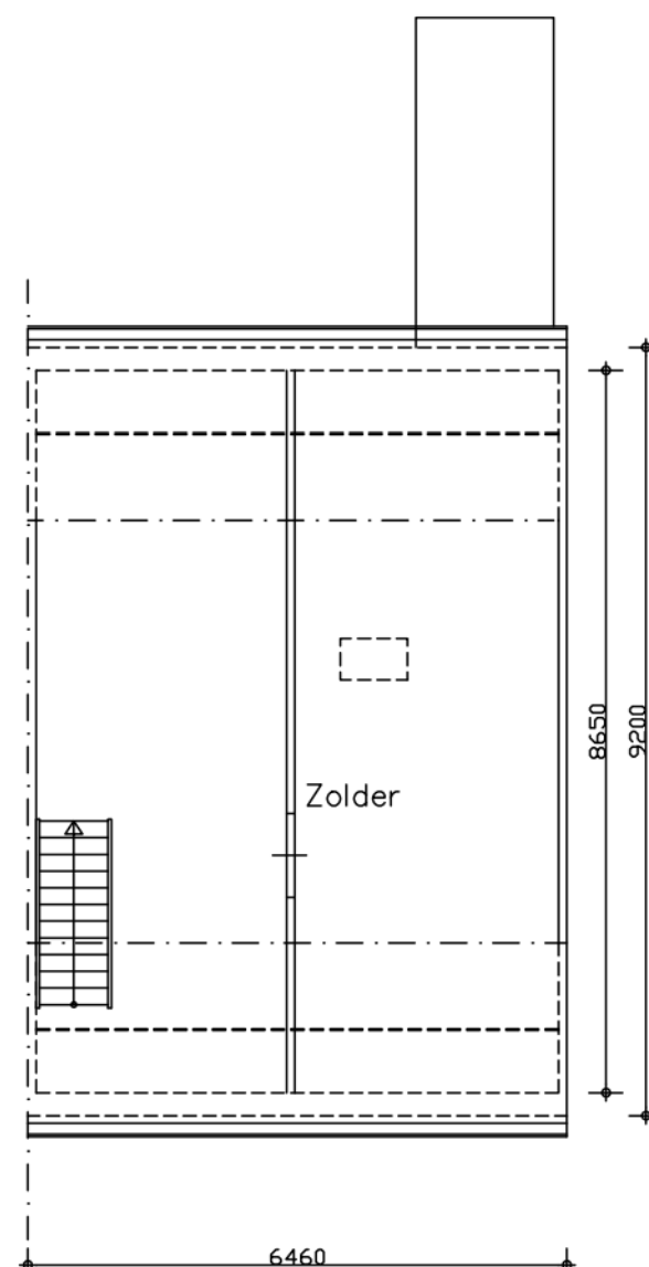
Zolder
