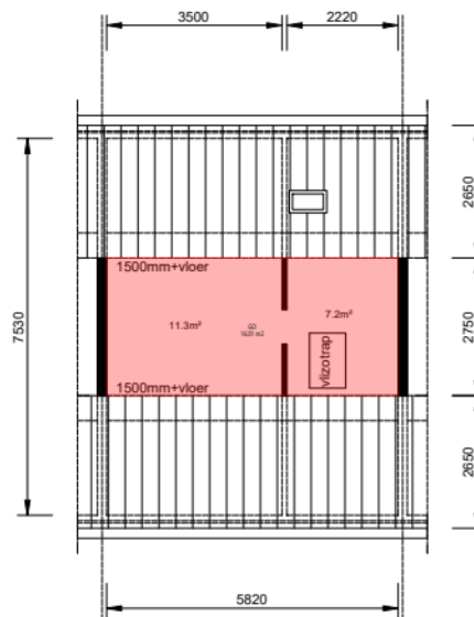
Zolder
