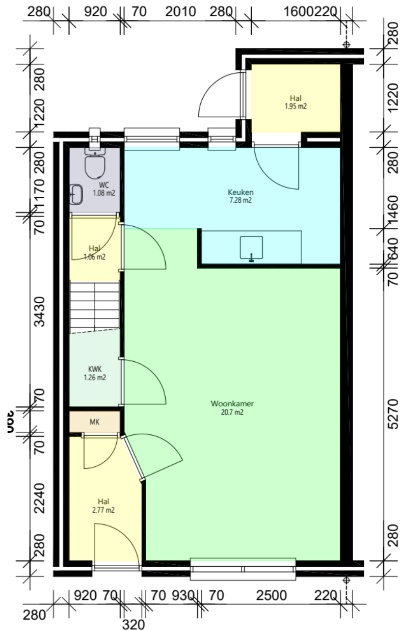
Begane_grond
