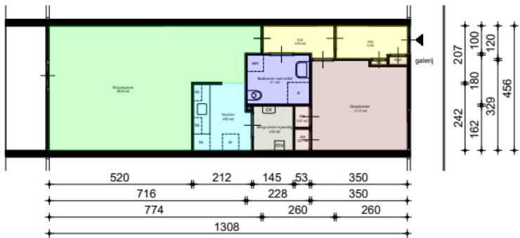
Begane_grond
