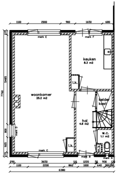
Begane-grond
