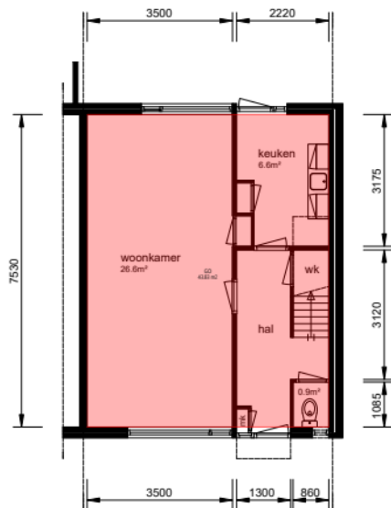
Begane_grond
