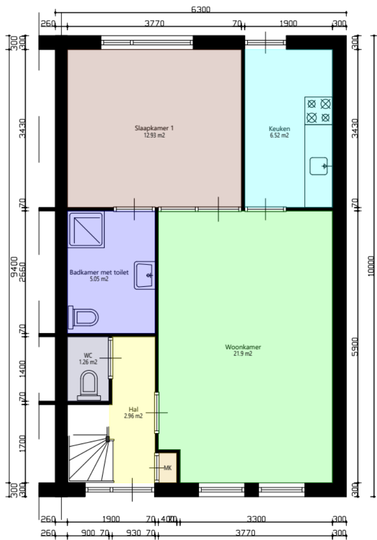
Begane_grond
