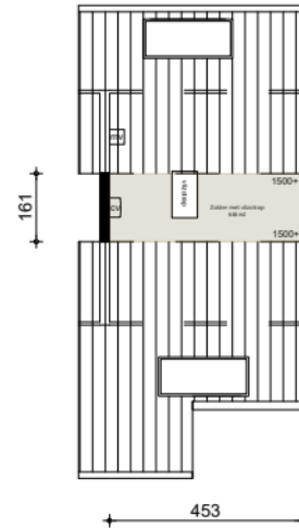
Zolder
