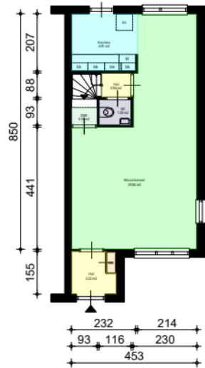
Begane_grond
