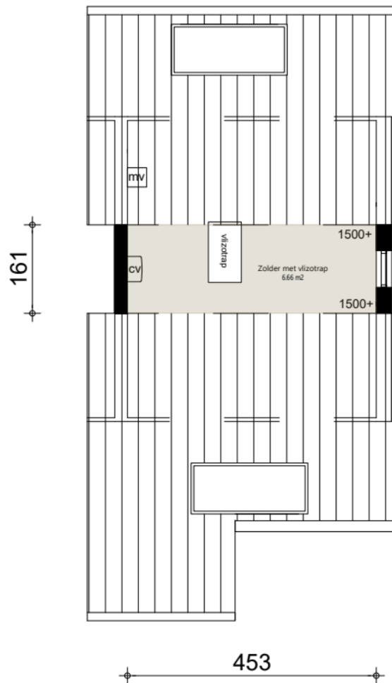
Zolder
