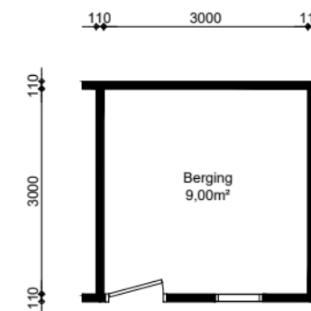
Berging
