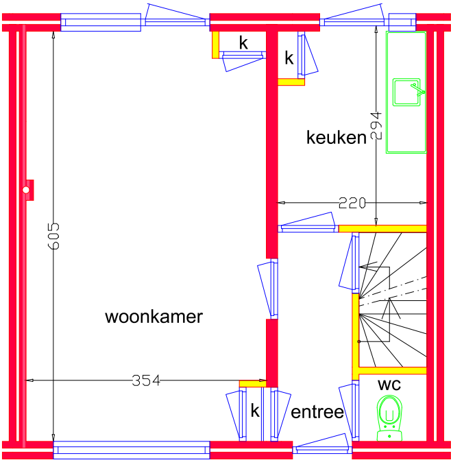
beganeground
