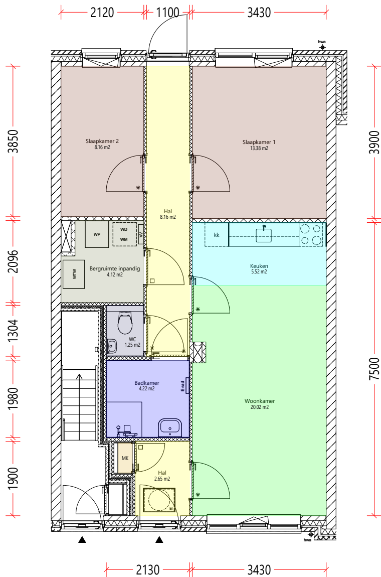
Begane_grond
