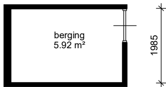
2980 begane grond
