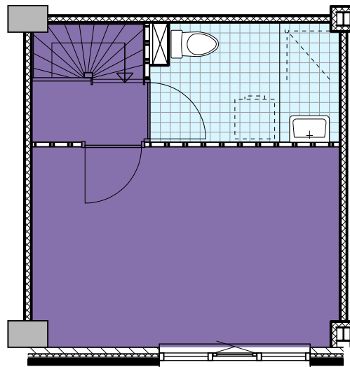
1e verdieping 1st floor
