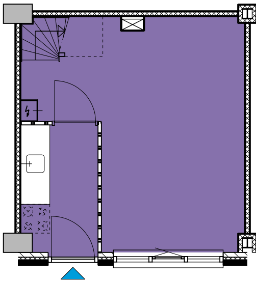
begane grond ground floor
