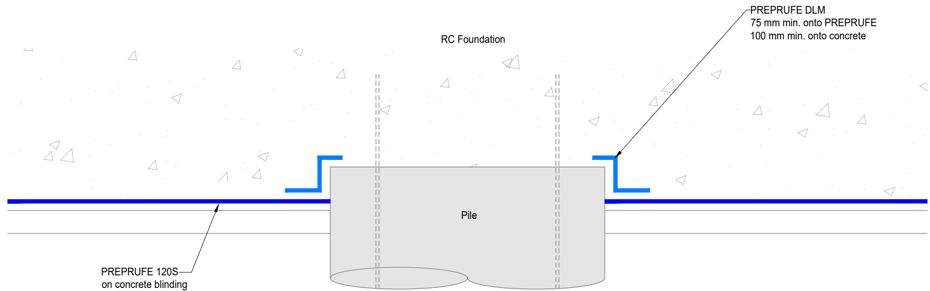
B PILE HEAD - PREPRUFE DLM Section
