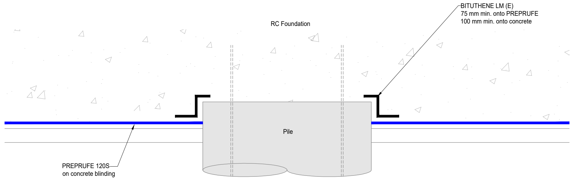
A PILE HEAD - BITUTHENE LM (E) Section
