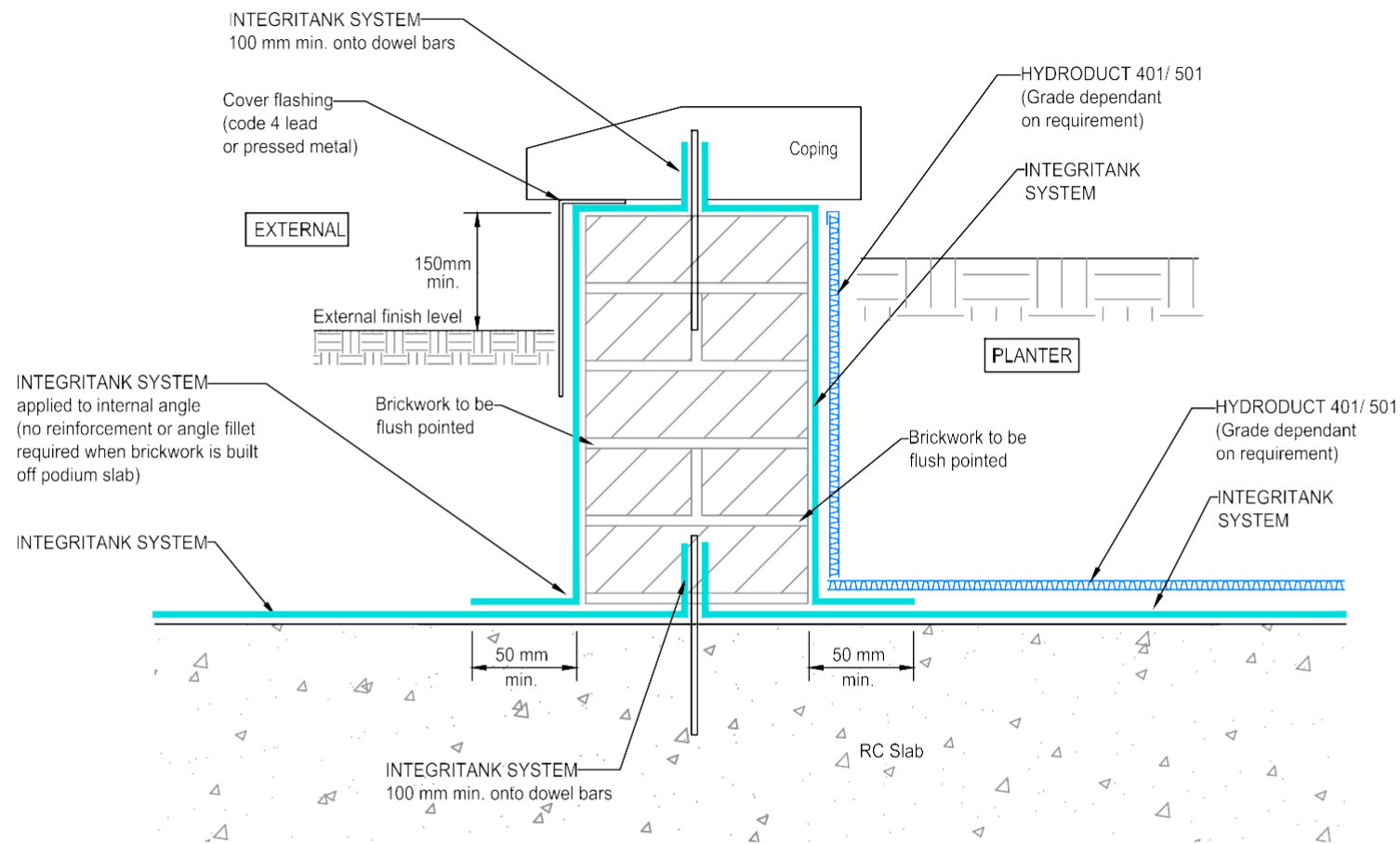
PLANTER DETAIL Section
